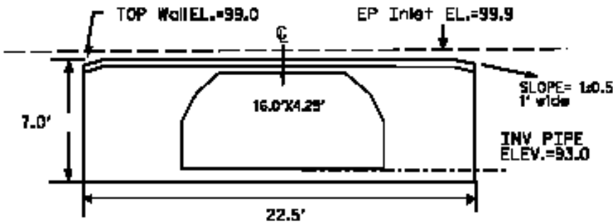
INLET
